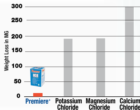
Steel Corrosion Damage Testing
